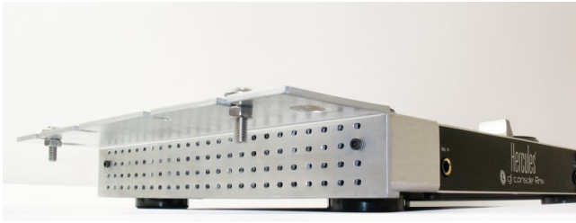
Rack ears
